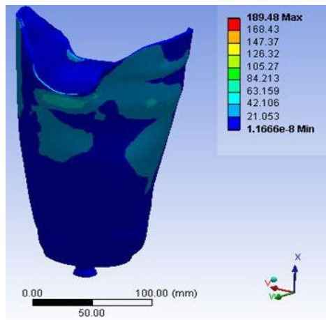
A. Stress Distribution without Temperature Effect
